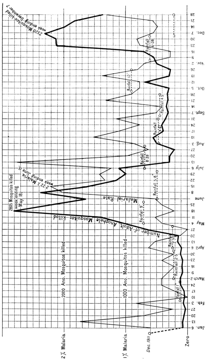
FIG. 45.—PANAMA. CHART OF THE MALARIA RATE AND MOSQUITO CATCH AT COROZAL. [Free page 204.]
