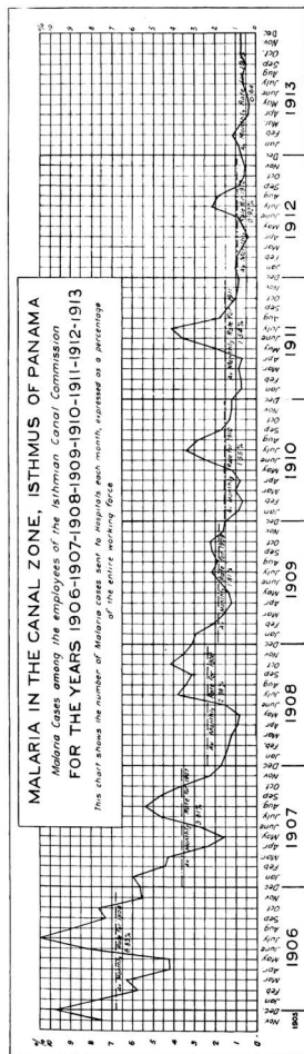
FIG. 48.—PANAMA. CHART OF MALARIA IN CANAL ZONE FROM 1906-1913.
